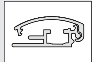
25mm profile with mitred corners.
